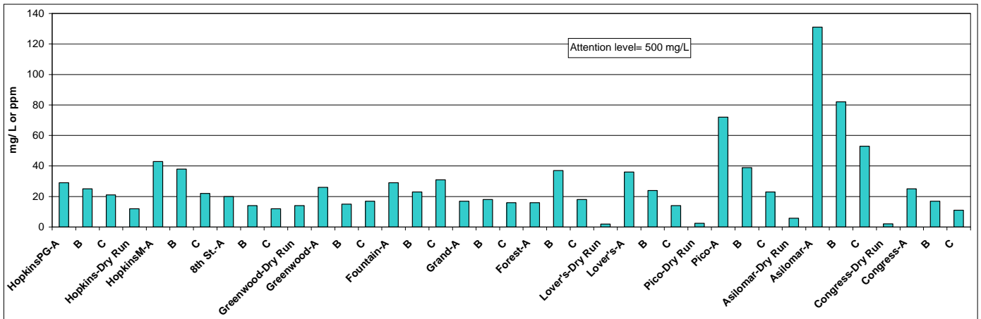
Figure 40. Total suspended solids (TSS) concentrations for the Dry Run and First Flush 2008 in Pacific Grove, CA.
